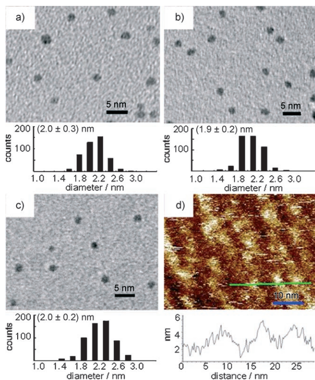
Figure 1. TEM images of \text{Au}_x(\text{SC}_6\text{H}_{13})_y and \text{Au}_x(\text{SC}_6\text{H}_{13})_y\text{-(S(CH}_2\text{CH}_2\text{O)}_3\text{CH}_3)_z : a) \text{Au}_x(\text{C}_6\text{H}_{13})_y before reprecipitation. b) \text{Au}_x(\text{SC}_6\text{H}_{13})_y reprecipitated from acetone/toluene (24:1). c) \text{Au}_x(\text{SC}_6\text{H}_{13})_y\text{-(S(CH}_2\text{CH}_2\text{O)}_3\text{CH}_3)_z . d) STM image of a Au electrode modified with \text{Au}_x(\text{SC}_6\text{H}_{13})_y\text{-(S(CH}_2\text{CH}_2\text{O)}_3\text{CH}_3)_z and the cross-sectional profile (green line in the STM image) along the cross-axis (bottom).
